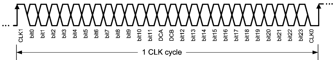
FIGURE 21. Single Serialized LVDS Bitstream*
