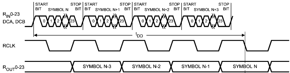
FIGURE 12. Deserializer Delay
