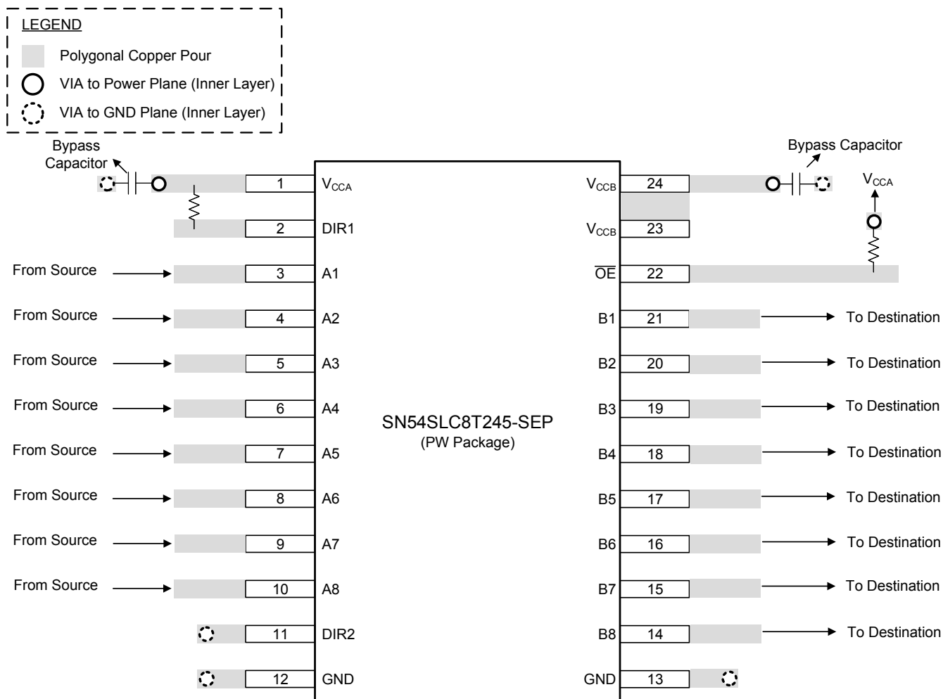
Figure 11-1. SN54SLC8T245-SEP Device Layout Example
