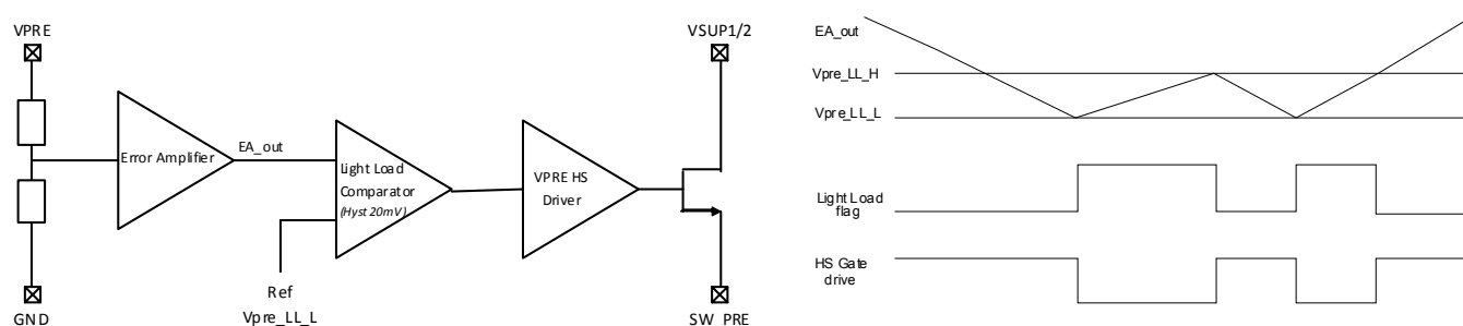
Figure 33. Description of light load condition
