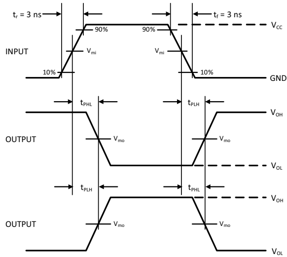
Figure 3. Switching Waveforms
