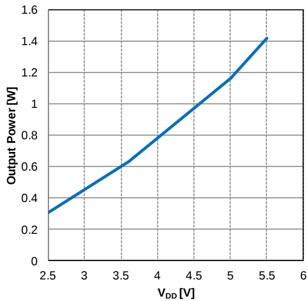
Figure 10. Output Power vs Power Supply (f=1kHz, R_L=8\Omega )
