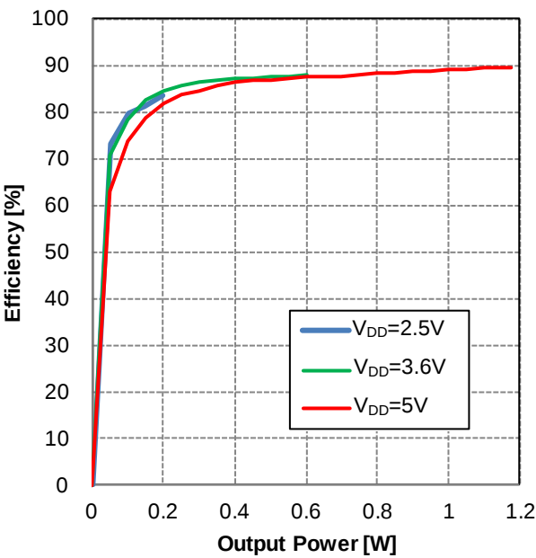
Figure 1. Efficiency vs Output Power (f=1kHz, R_L=8\Omega+33\mu\text{H} )
