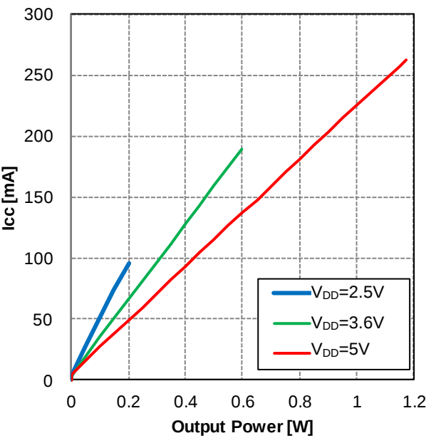
Figure 3. Supply Current vs Output Power (f=1kHz, R_L=8\Omega+33\mu\text{H} )
