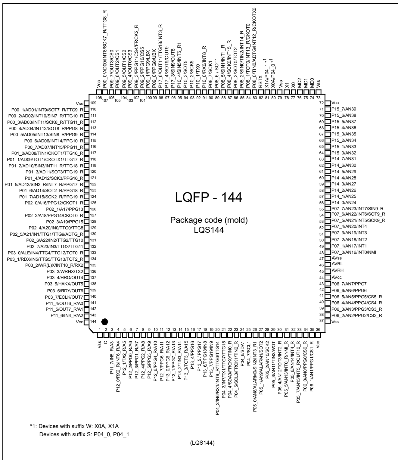
Pin assignment of CY96F33xY/R (LQS144)
