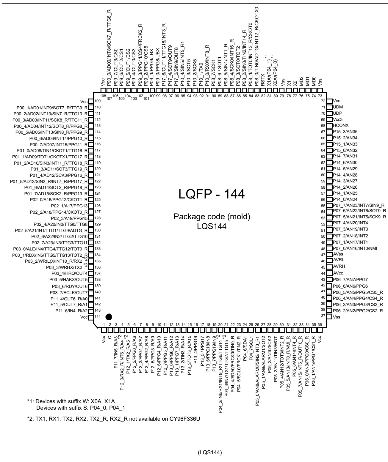
Pin assignment of CY96F33xU (LQS144) USB device
