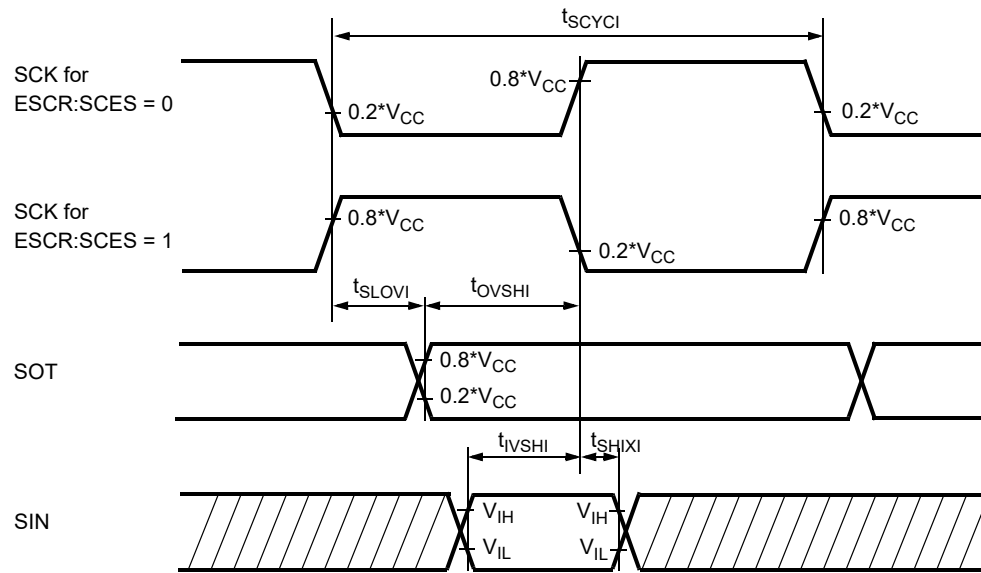
Internal Shift Clock Mode
