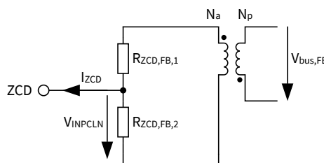
Figure 24 Bus Voltage Sensing using ZCD Clamp Current
