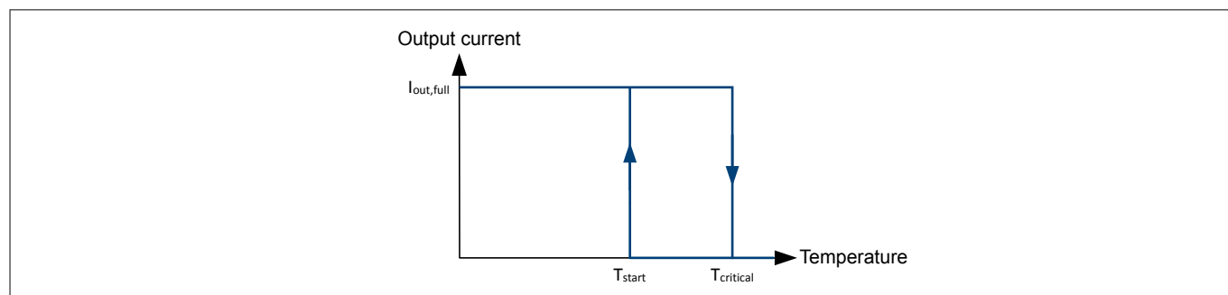
Figure 29 Temperature protection
