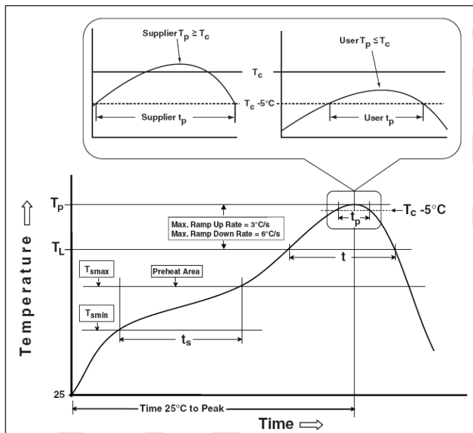
Figure 27 Classification Profile
