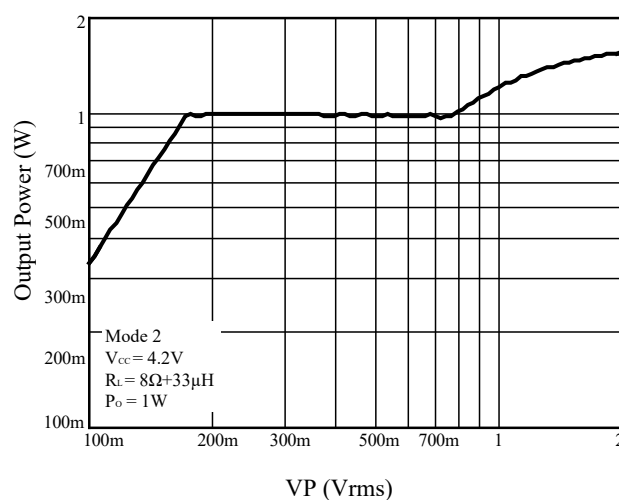
Figure 8 Output Power vs. VP
