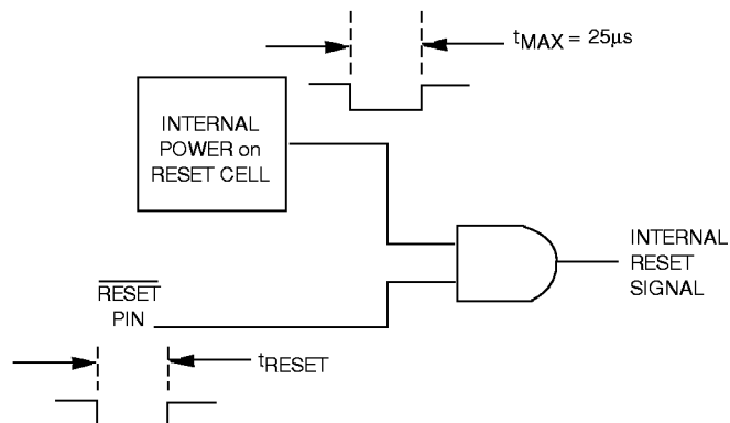
Fig. 10 Reset Circuitry
