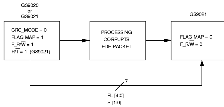
Fig. 6b Example of FLAG_MAP Mode Implementation
