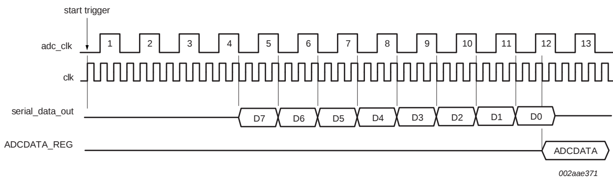
Fig 35. ADC conversion timing
