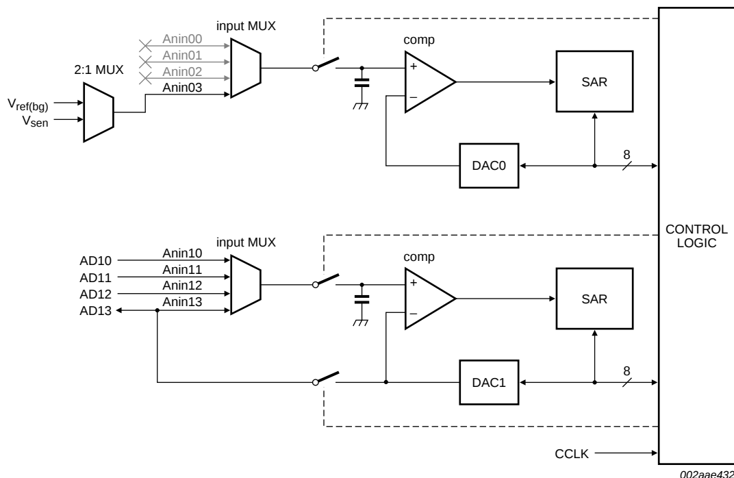
Fig 15. ADC block diagram
