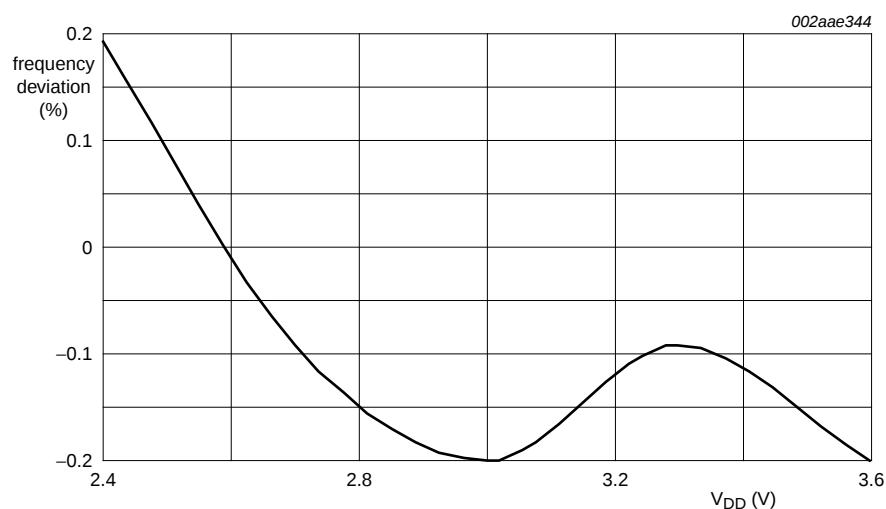
Fig 25. Average internal RC oscillator frequency vs. V_{DD} at +25 °C
