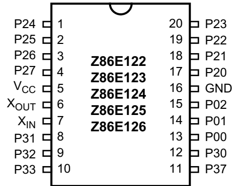
Figure 2. 20-Pin DIP/SOIC Pin Configuration
