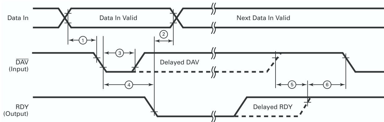
Figure 27. Input Handshake Timing
