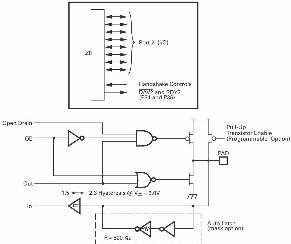
Figure 12. Port 2 Configuration
