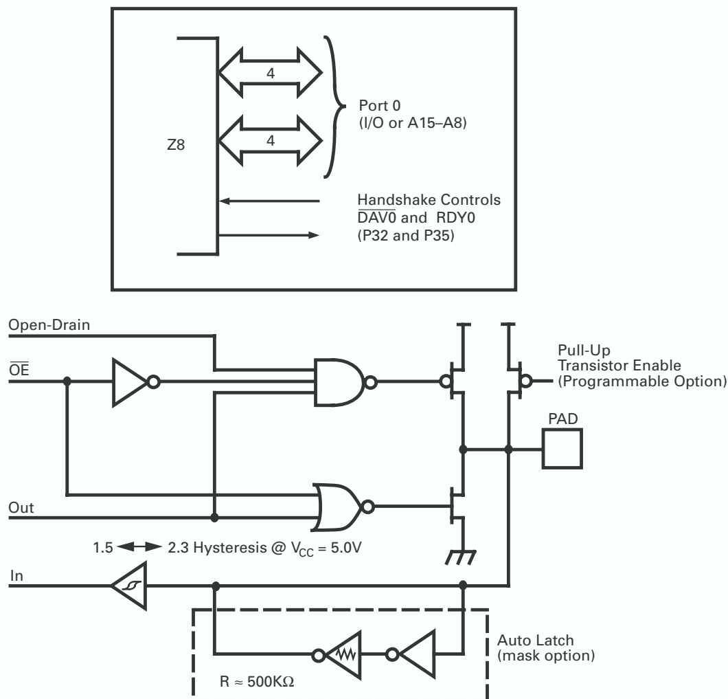
Figure 10. Port 0 Configuration
