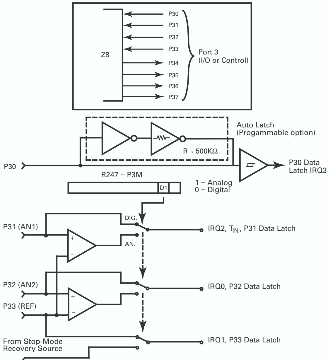
Figure 13. Port 3 Configuration
