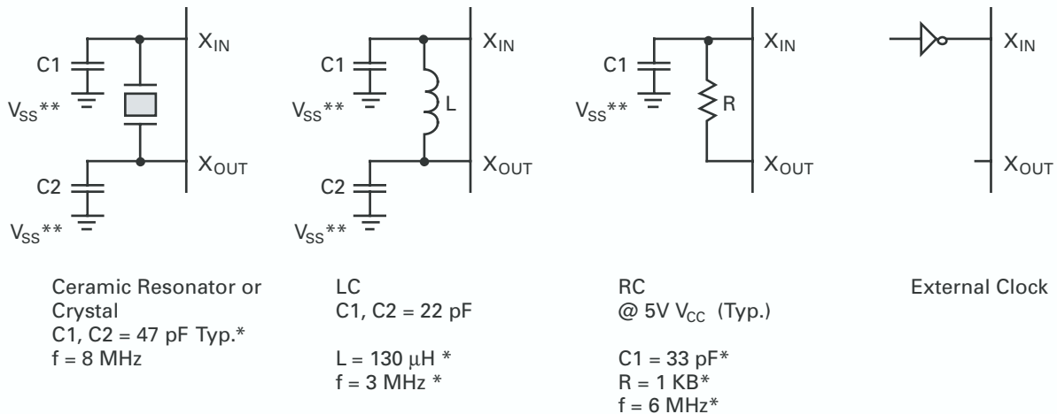
Figure 20. Oscillator Configuration
