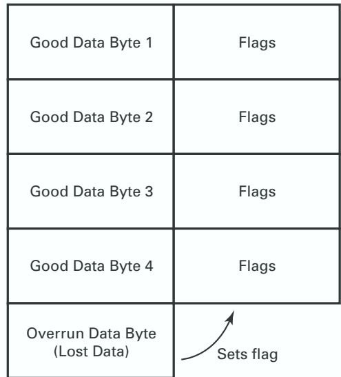
Figure 31. FIFO Overflow Example
