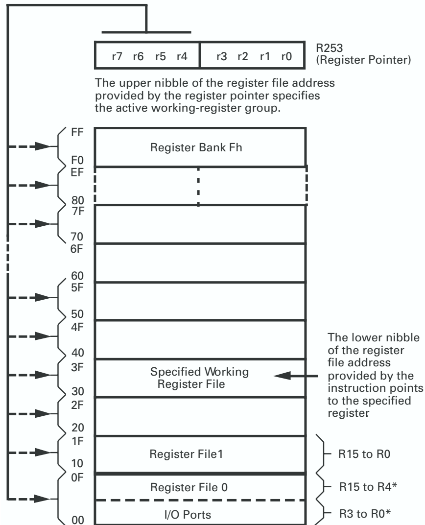
Figure 17. Register Pointer—Detail
