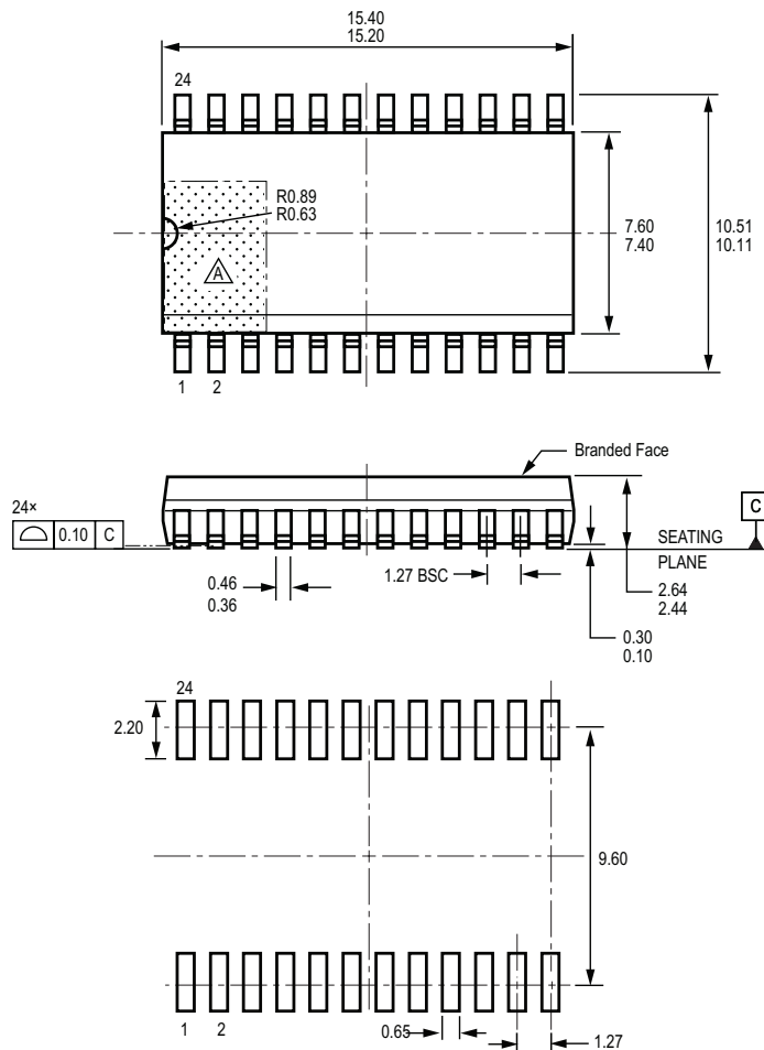
B PCB Layout Reference View
