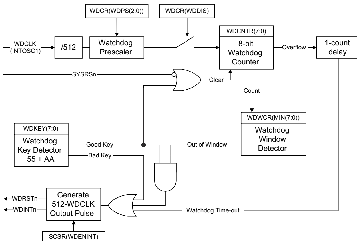
Figure 8-4. Windowed Watchdog
