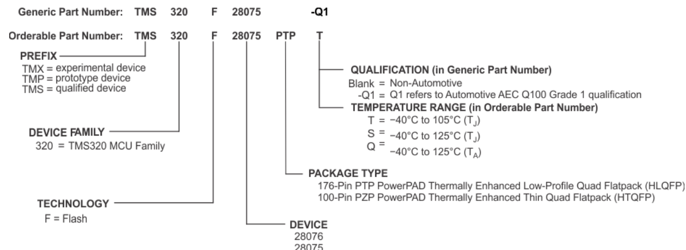
Figure 10-1. Device Nomenclature
