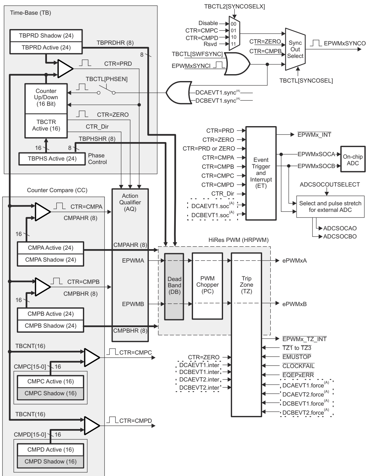
Figure 7-45. ePWM Submodules and Critical Internal Signal Interconnects
