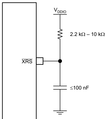
Figure 7-4. Reset Circuit
