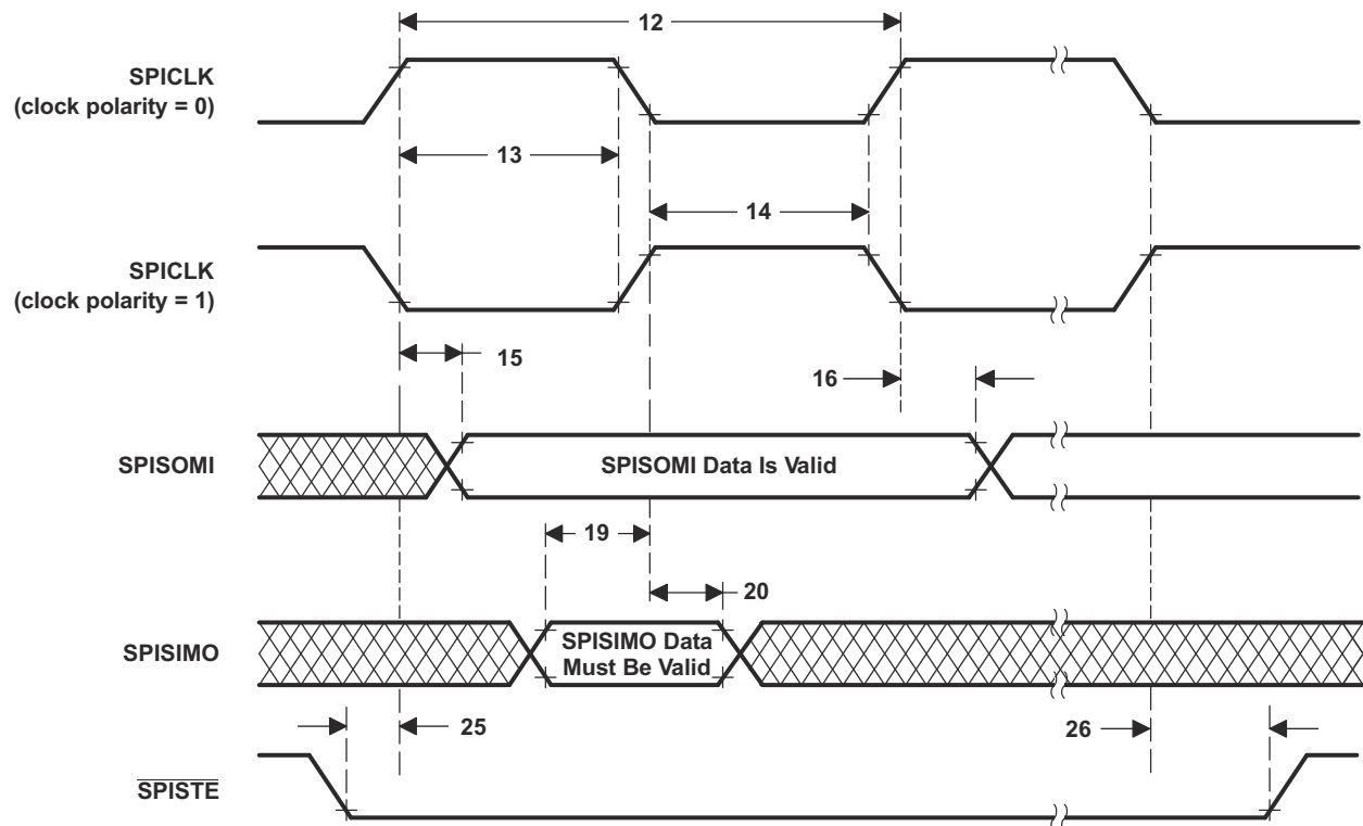
Figure 7-70. SPI Slave Mode External Timing (Clock Phase = 0)
