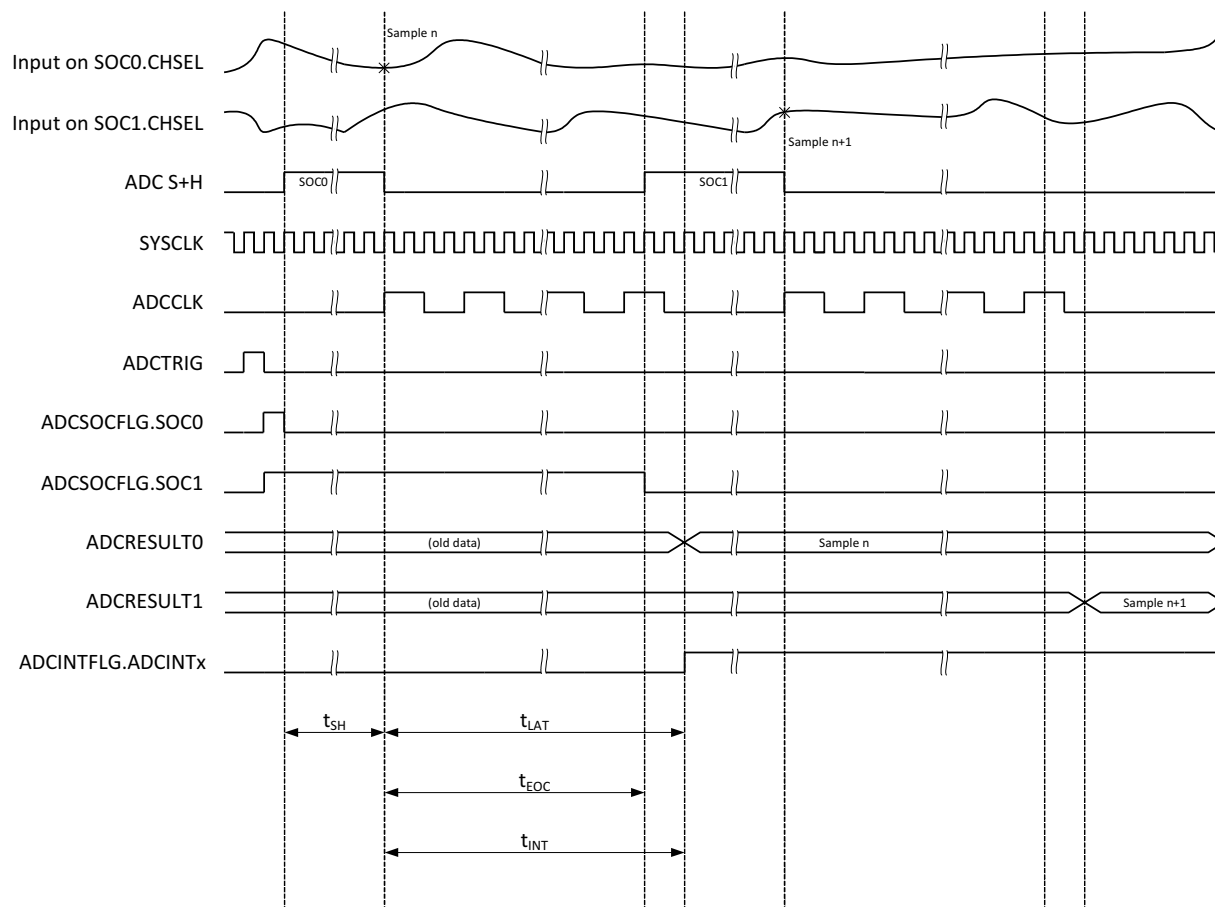
Figure 7-32. ADC Timings for 12-Bit Mode
