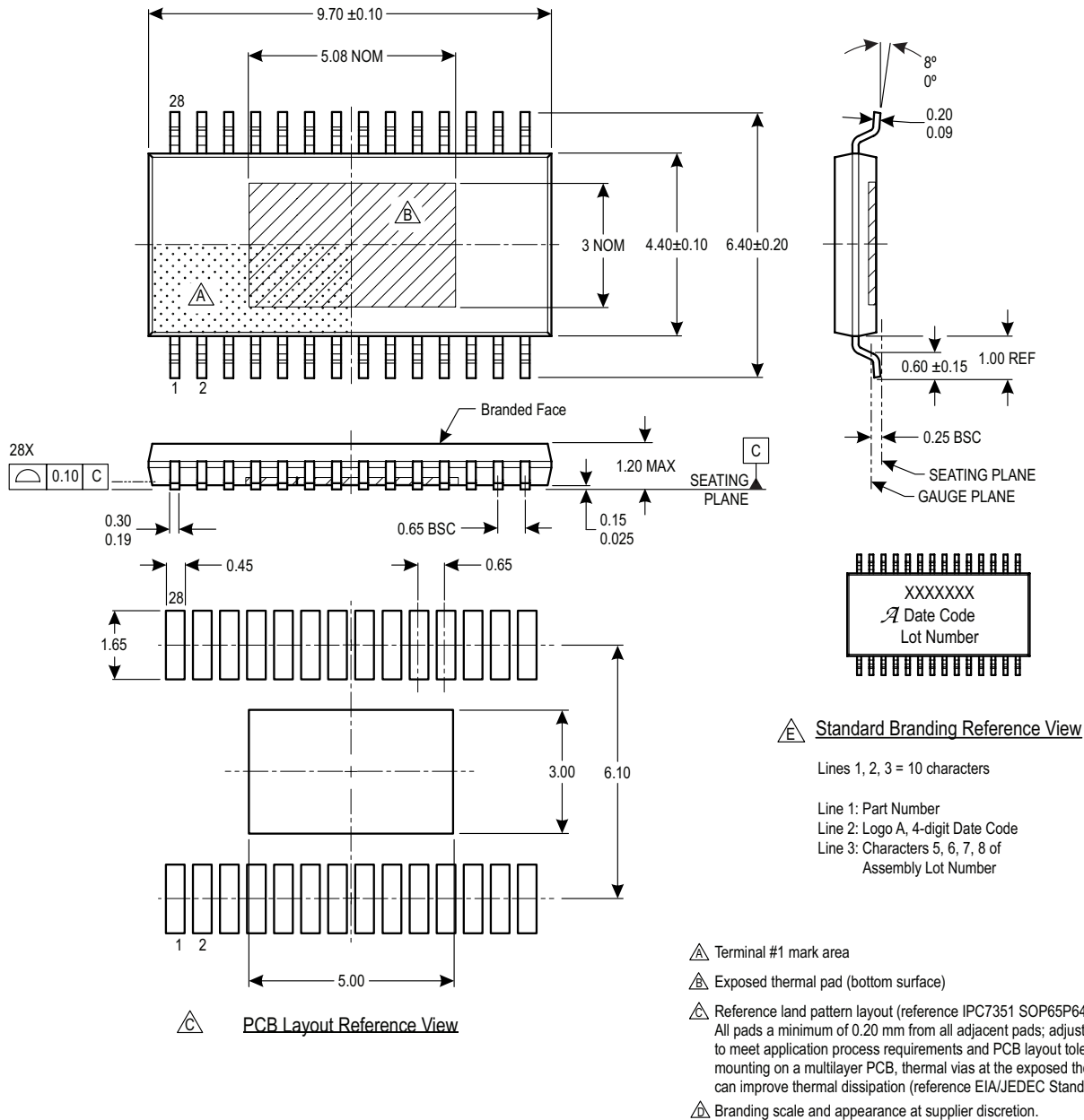
Figure 20: Package LP, 28-Pin TSSOP with Exposed Thermal Pad
