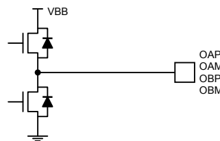
Figure 19i: Phase Outputs
