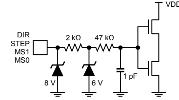
Figure 19c: DIR, STEP, MS1, MS0 Inputs
