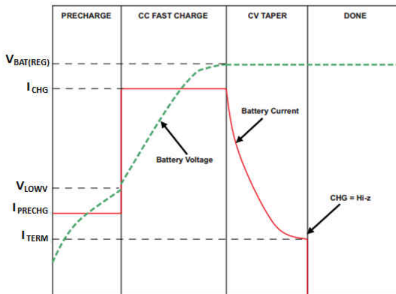
Figure 9-2. BQ21062 Typical Charge Cycle
