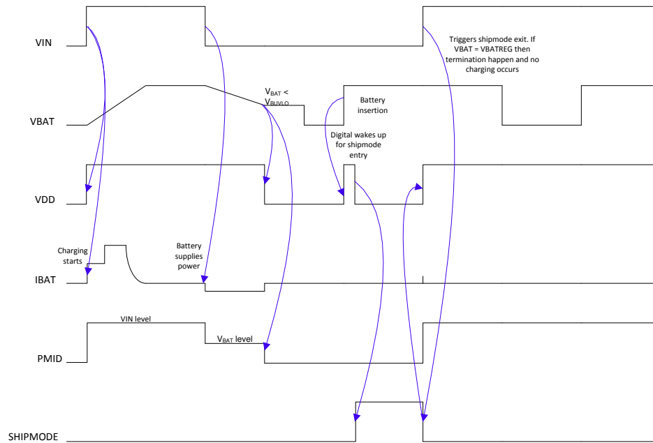
Figure 9-14. BQ21062 Wake-Up Upon Supply Insertion
