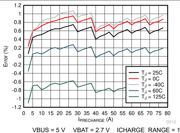
Figure 8-4. Pre-Charge Current Accuracy vs. IPRECHARGE Setting (ICHARGE_RANGE = 1)
