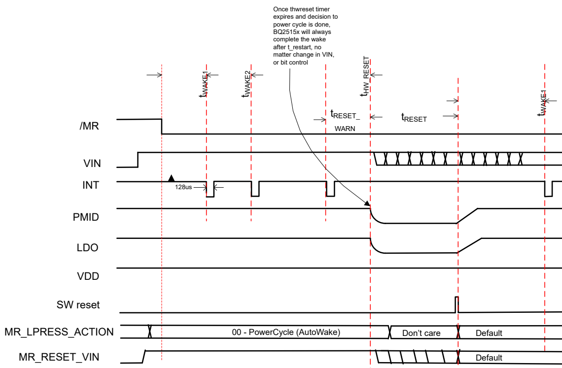
Figure 9-5. MR Wake and Reset Timing with VIN Present or BAT Active Mode When MR\_LPRESS\_ACTION = 00
