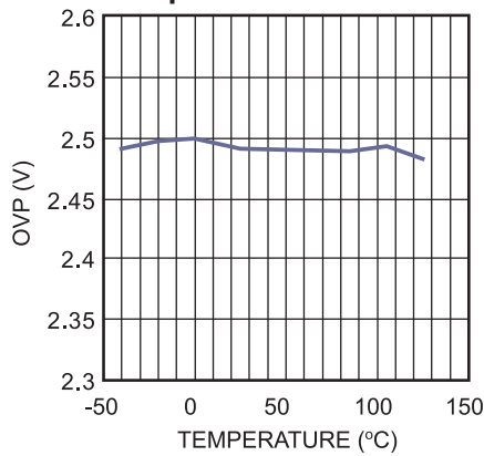
OVP Protection Point vs. Temperature
