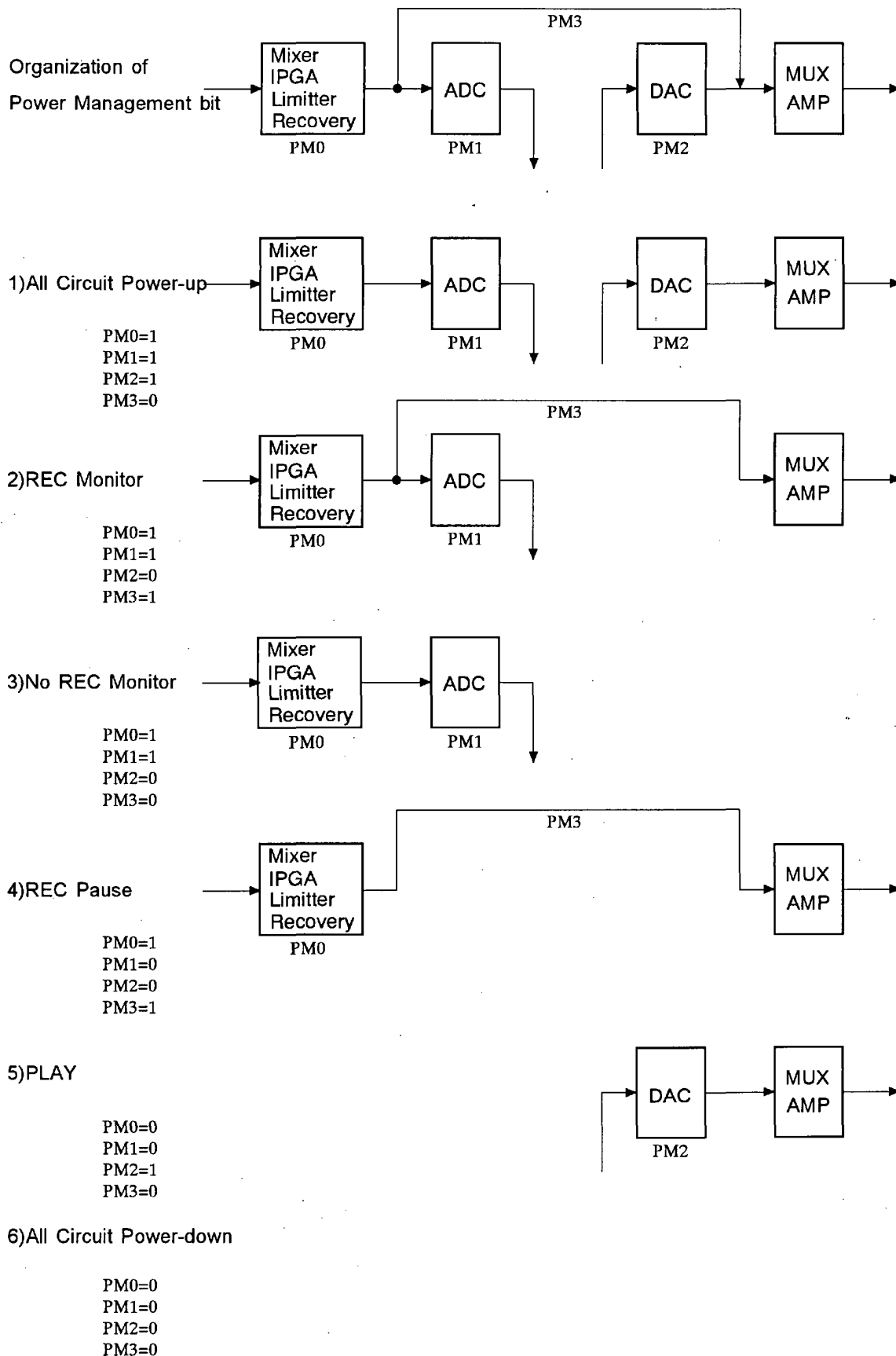
Figure 11 . Power Management
