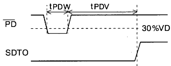
Reset Timing
