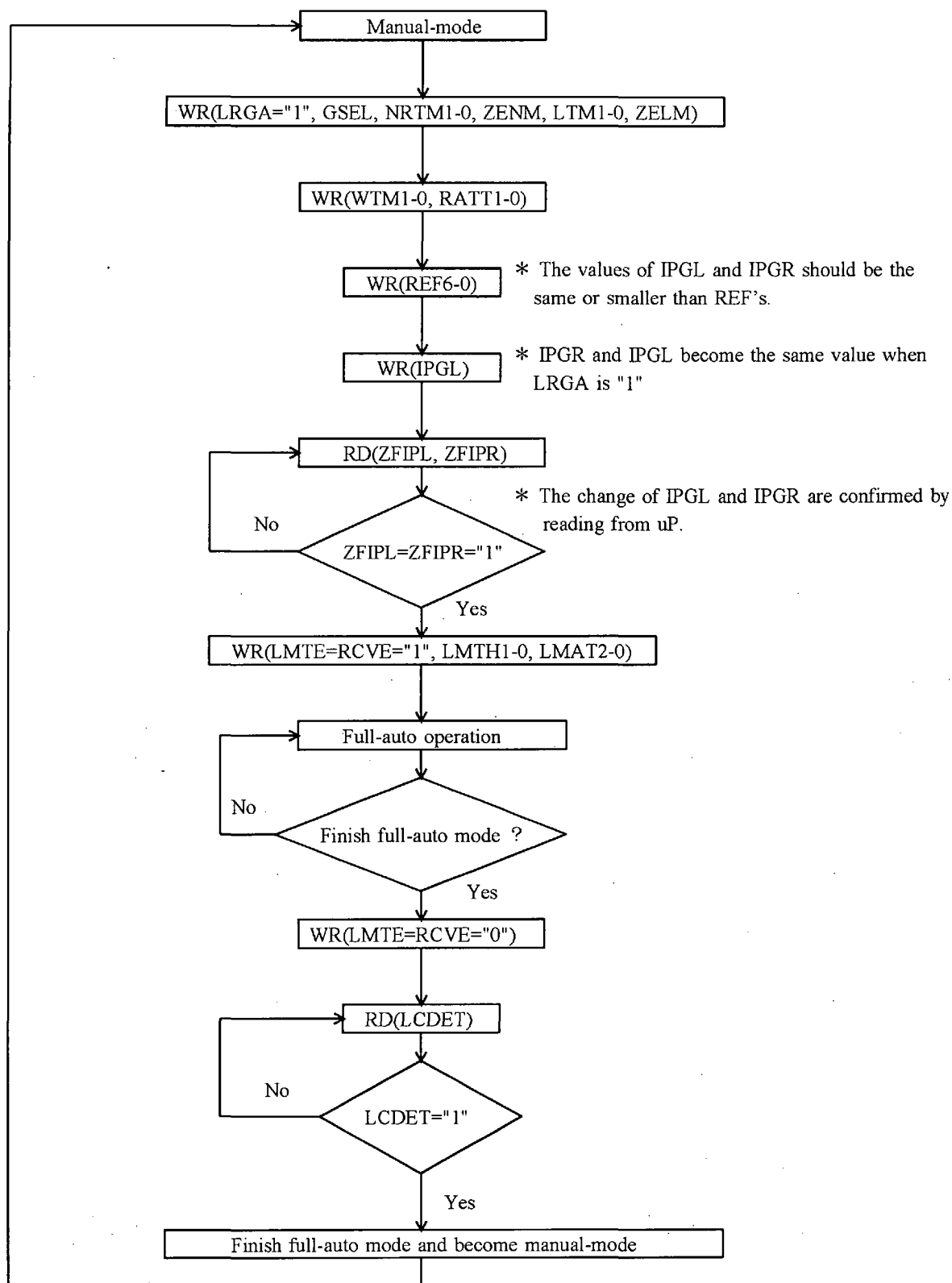
Figure 10 . Registers set-up sequence at Full-auto mode
