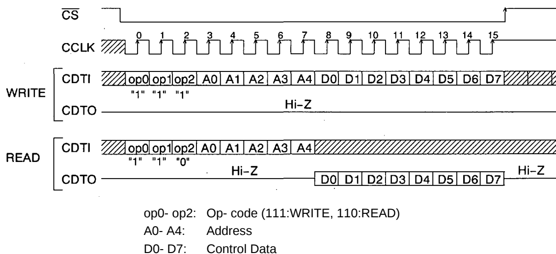
Figure 5 . Control Data Timing
