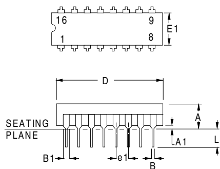
16 pin Plastic DIP
