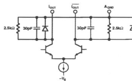
Output Circuit
