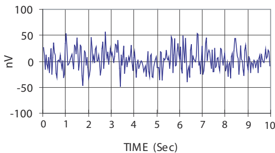
Figure 3. 0.01 Hz to 10 Hz Noise
