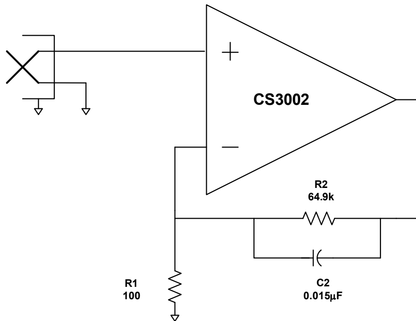
Figure 17. Thermopile Amplifier with a Gain of 650V/V
