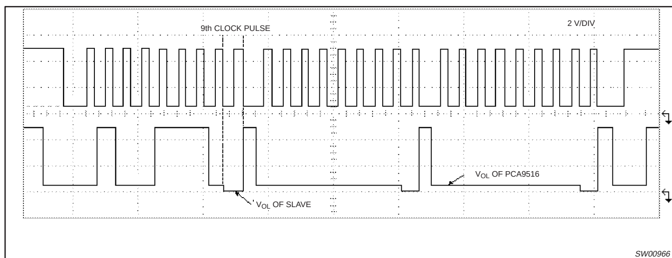
Figure 6. Bus 1 waveform
