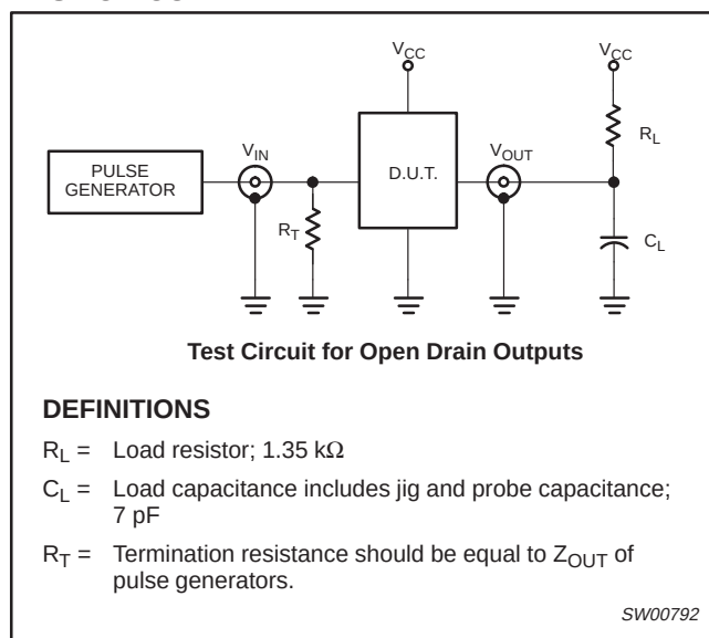
Figure 7. Test circuit
