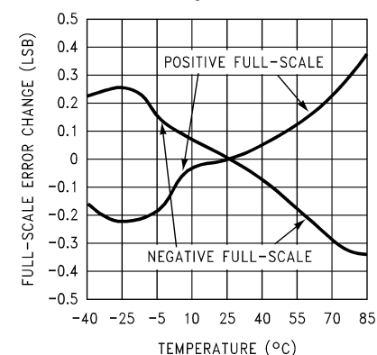
Full-Scale Error Change vs. Temperature
