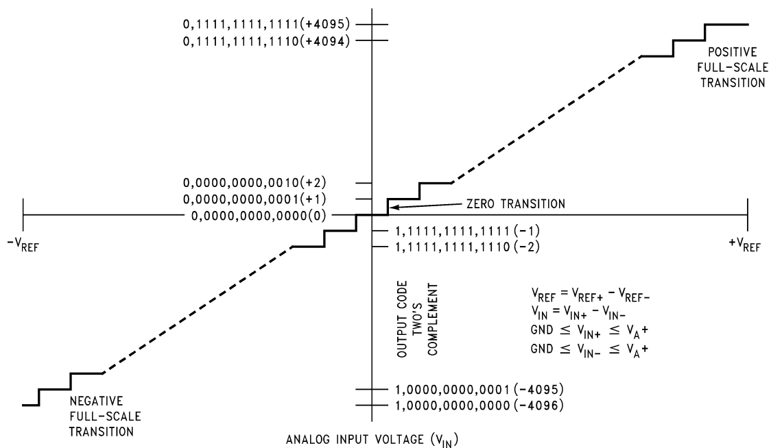
FIGURE 6. Transfer Characteristic
