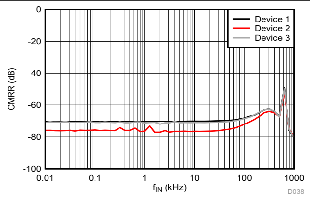
Figure 6-28. Common-Mode Rejection Ratio vs Input Frequency
