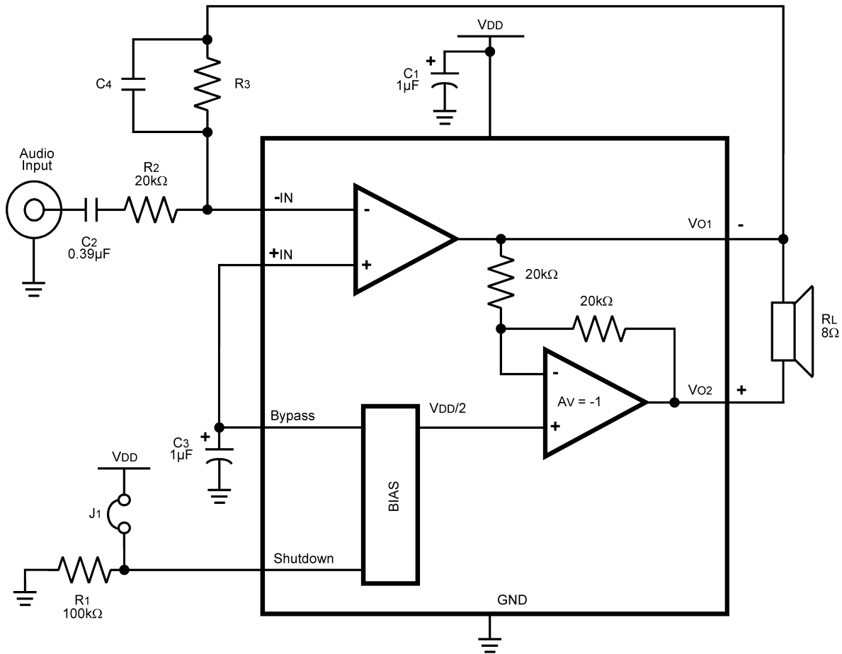
FIGURE 2. HIGHER GAIN AUDIO AMPLIFIER
