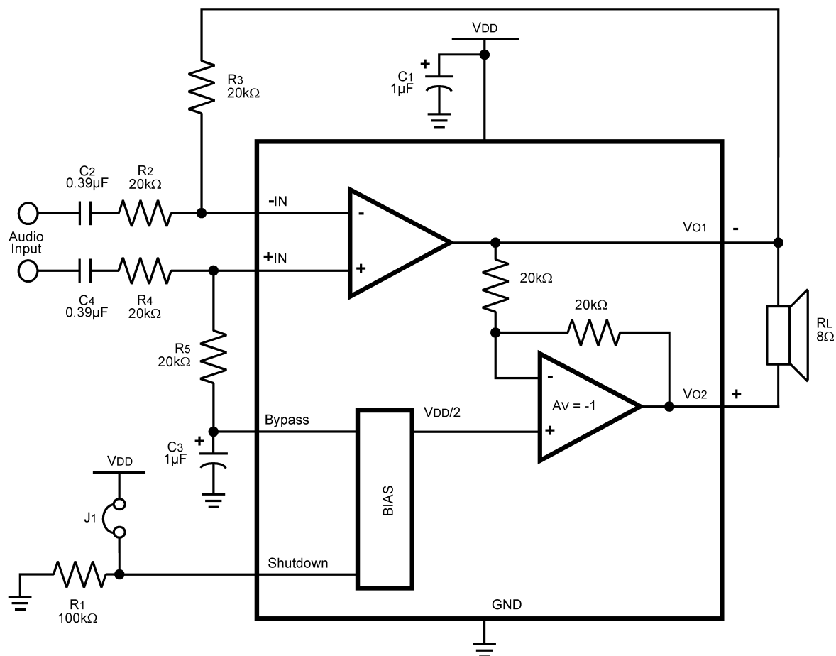
FIGURE 3. DIFFERENTIAL AMPLIFIER CONFIGURATION FOR LM4904
