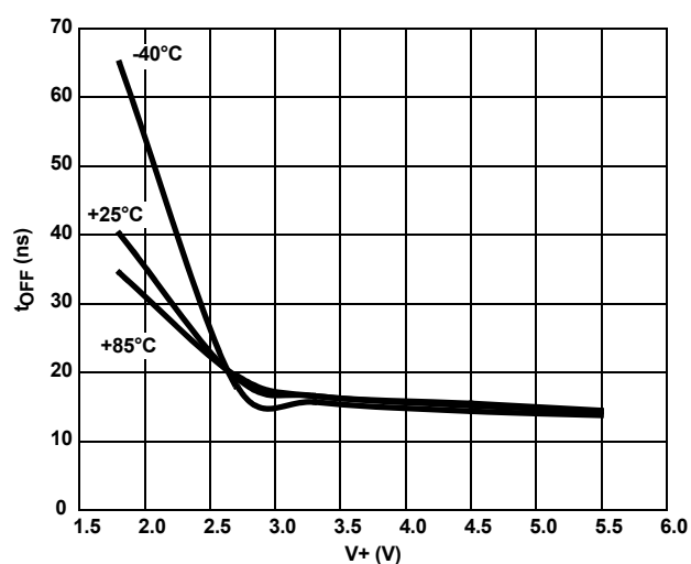
FIGURE 13. TURN-OFF TIME vs SUPPLY VOLTAGE
