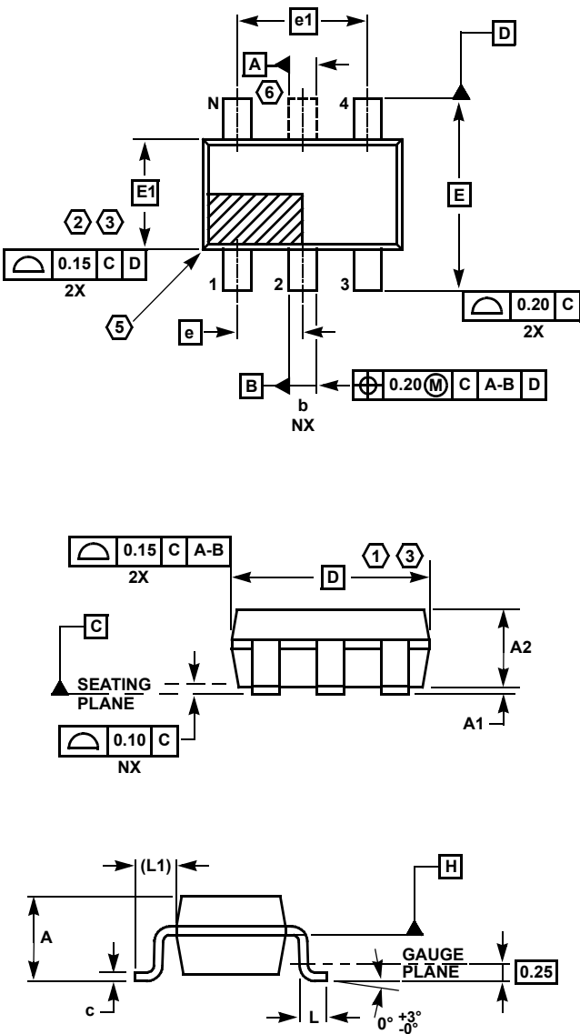
MDP0038 SOT-23 PACKAGE FAMILY
