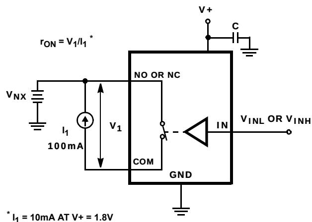
FIGURE 4. r_{ON} TEST CIRCUIT
