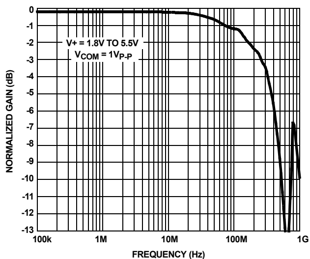
FIGURE 15. FREQUENCY RESPONSE
