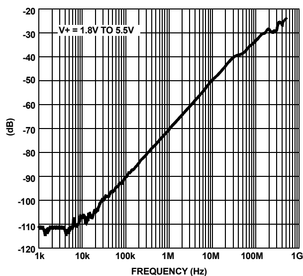
FIGURE 16. OFF ISOLATION
