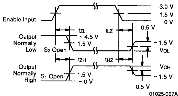
Enable And Disable Times (Notes 2 and 3)
