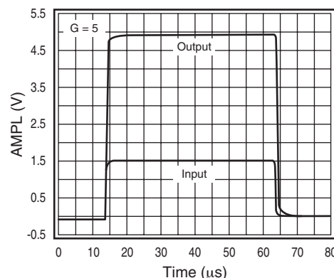
Figure 3: Overdrive Recovery
