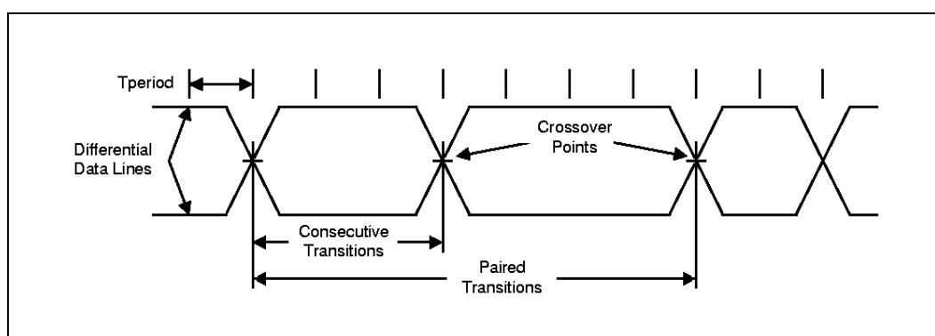
Figure 14-14. USB Jitter
