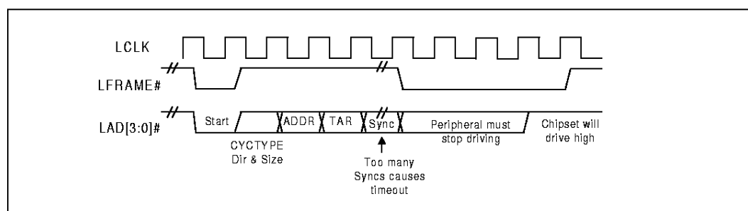
Figure 5-6. Abort Mechanism
