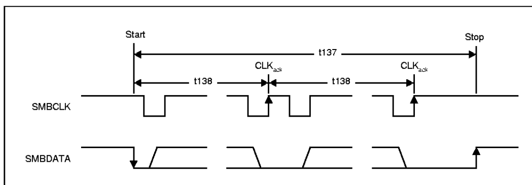
Figure 14-17. SMBus Timeout
