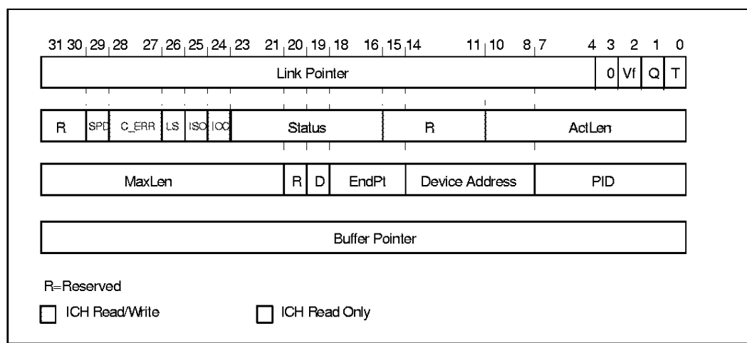
Figure 5-13. Transfer Descriptor
