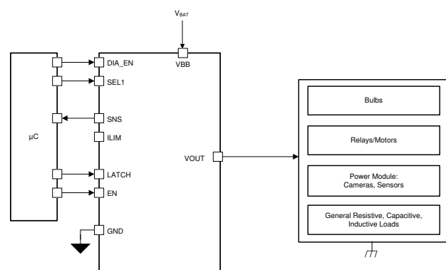
Simplified Schematic
