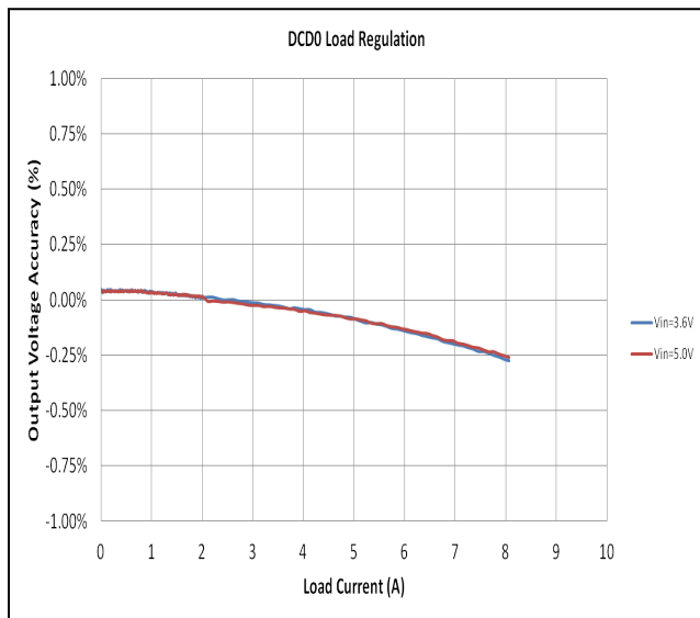
Figure 4. Load Regulation
