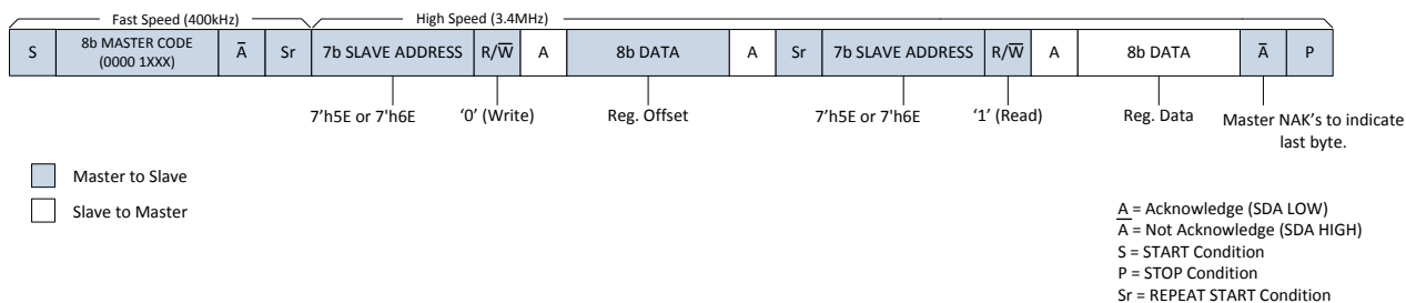
Figure 40: I2C High Speed Read
