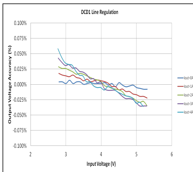
Figure 9. Line Regulation
