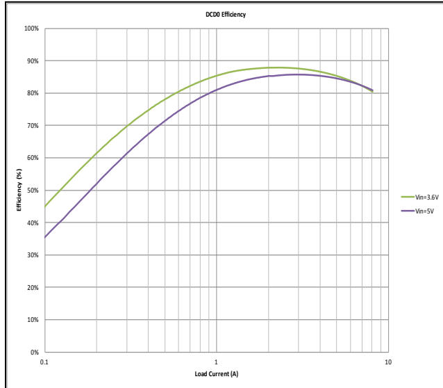
Figure 2. Efficiency
