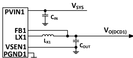
Figure 26. DCD1 External component connections
