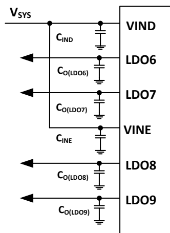
Figure 32. LDO6,7,8,9 External component connections
