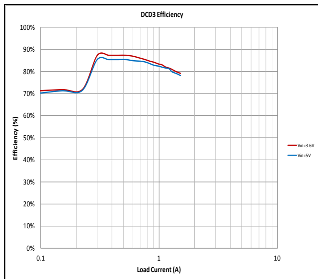
Figure 14. Efficiency
