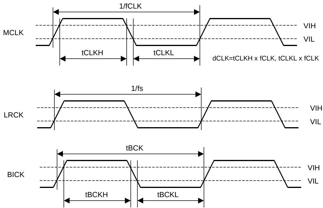
Clock Timing
