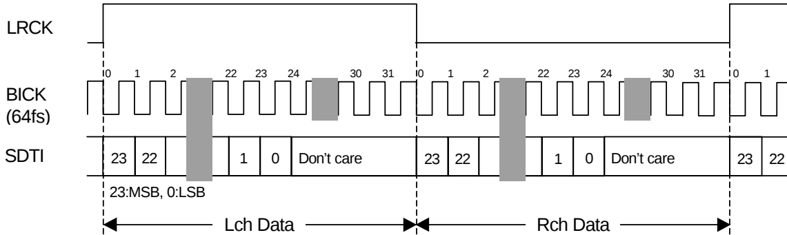
Figure 3. Mode 2 Timing
