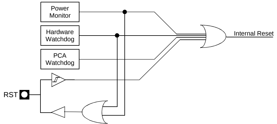
Figure 69. Reset schematic
