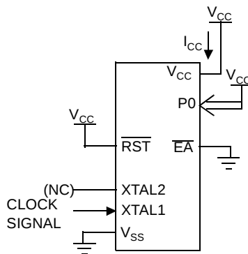
Figure 76. I_{CC} Test Condition, Idle Mode
