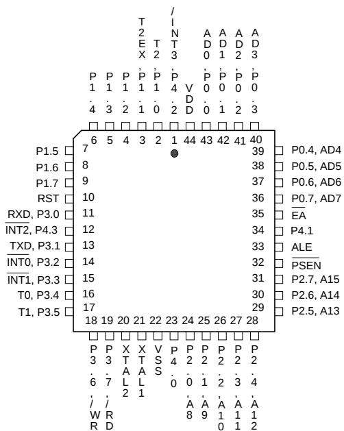
44-Pin PLCC
