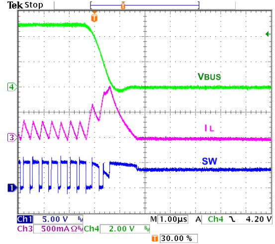
Figure 30. V_{BUS} Fault Response, 3.6\text{ V}_{BAT}
