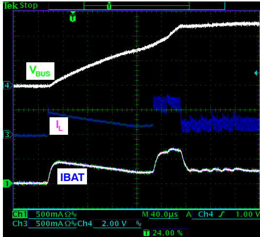
Figure 29. Startup, 3.6\text{ V}_{BAT} , 44\ \Omega Load, Additional 10\ \mu\text{F} , X5R Across V_{BUS}
