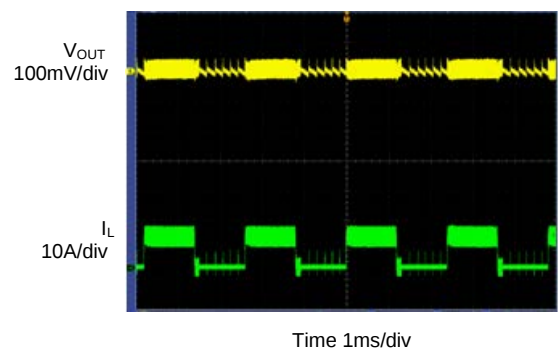
Load Transient Response @ DEM
