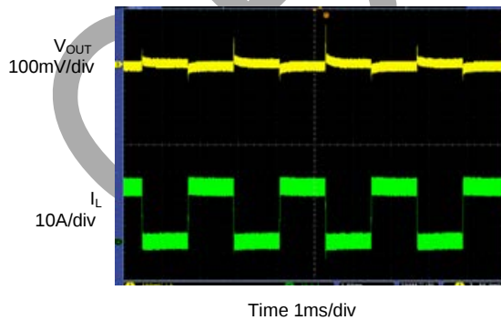
Load Transient Response @ CCM
