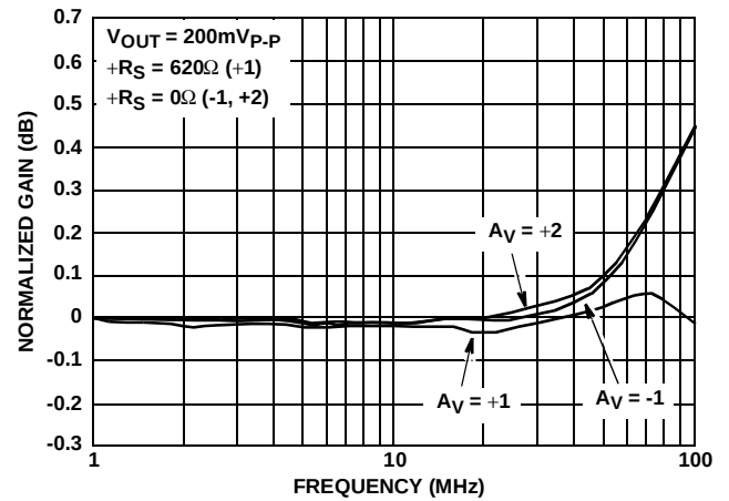
FIGURE 15. GAIN FLATNESS
