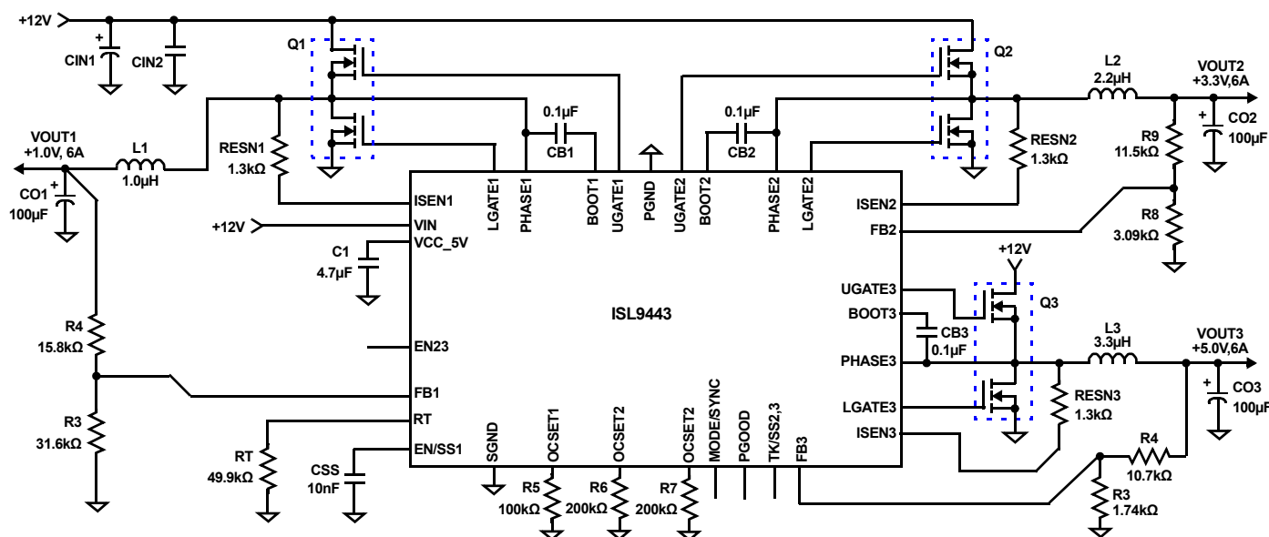
FIGURE 1. TYPICAL APPLICATION
