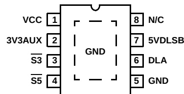
ISL6506 (8 LD EPDIP) TOP VIEW
