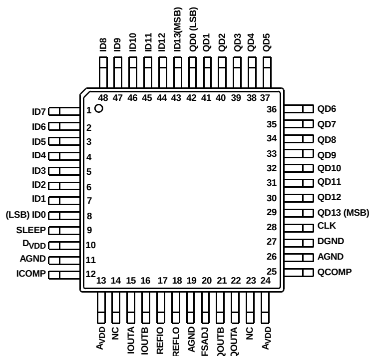
ISL5929 (LQFP) TOP VIEW
