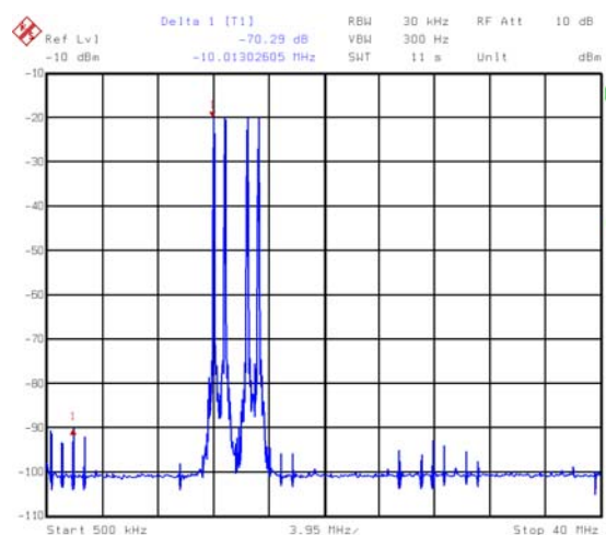
FIGURE 12. FOUR TONES (CF=8.1) AT 14MHz, 80MSPS CLOCK, 800kHz SPACING (70dBc - NYQUIST, 6dB PAD)
