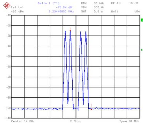
FIGURE 6. FOUR GSM CARRIERS AT 12.4–15.6MHz, 800kHz SPACING, 78MSPS (75+dBc - 20MHz WINDOW, 6dB PAD)
