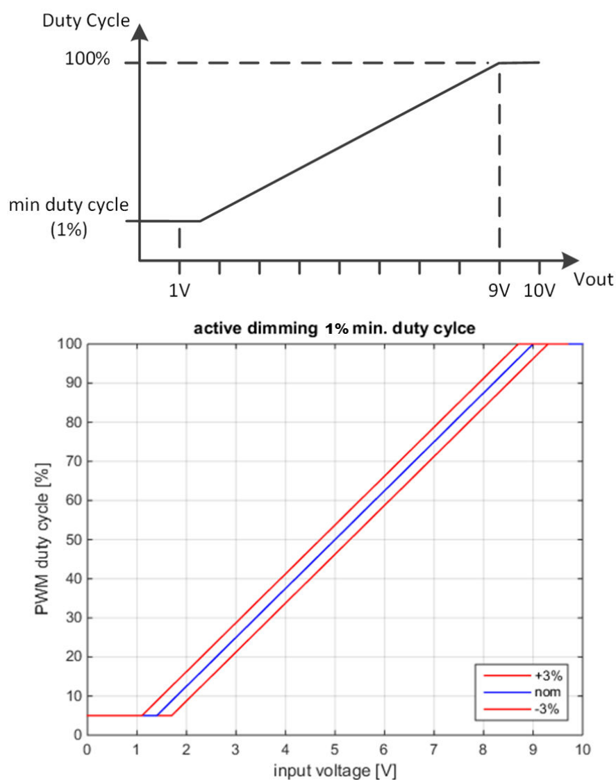
Figure 4 Dimming Characteristic
