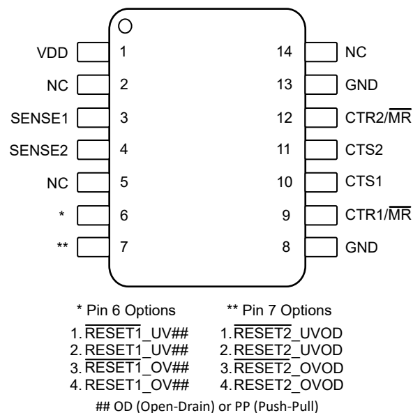
Figure 6-2. DYY Package, 14-Pin SOT-23, TPS38 (Top View) PRODUCT PREVIEW
