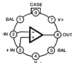
HA2-5180 (TO-99 METAL CAN) TOP VIEW
