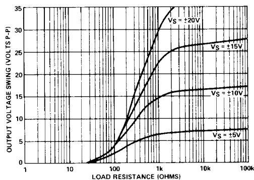
OUTPUT VOLTAGE SWING vs. LOAD RESISTANCE
