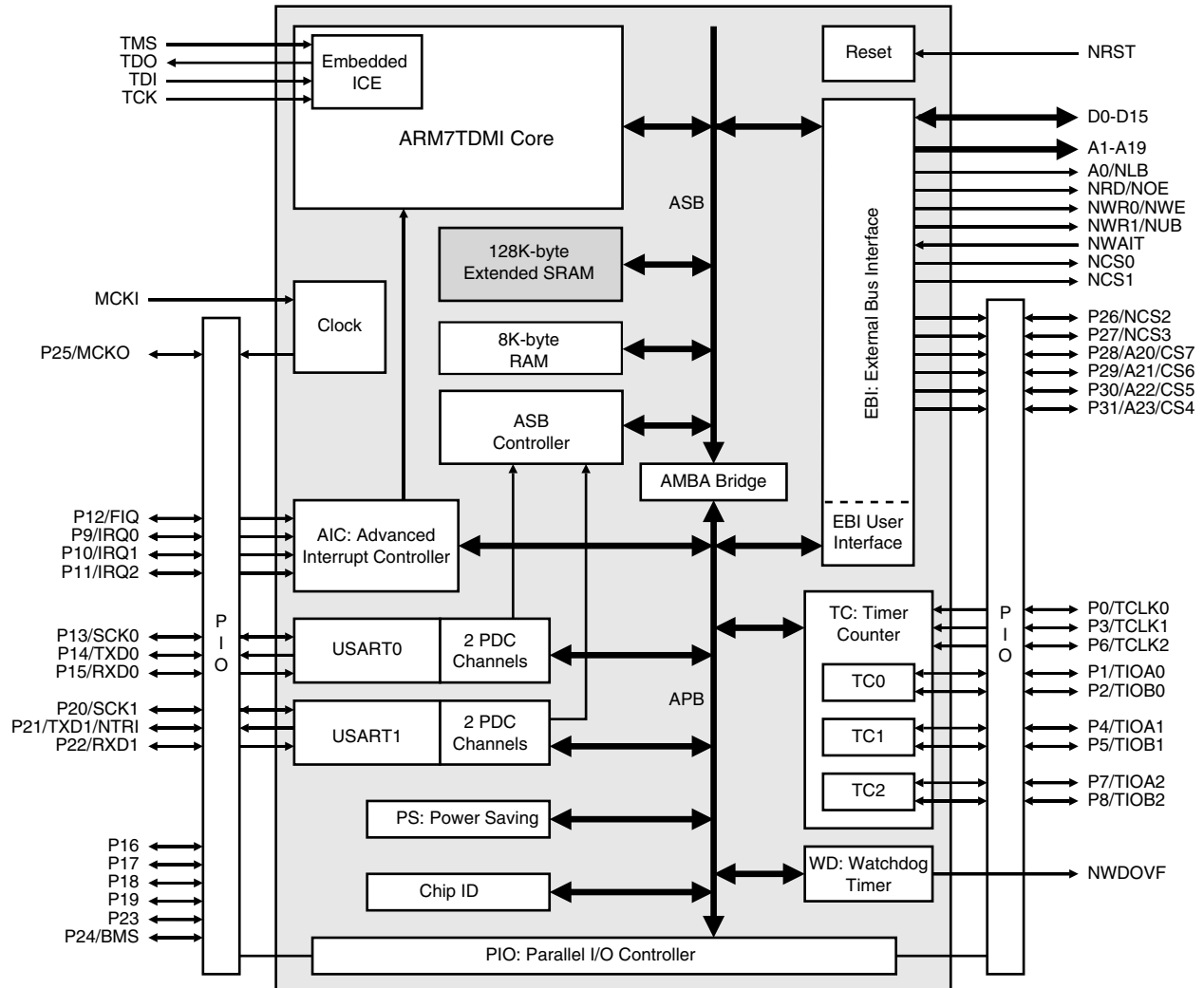
Figure 2. AT91R40807
