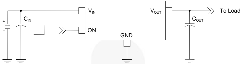
Figure 2. Typical Application
