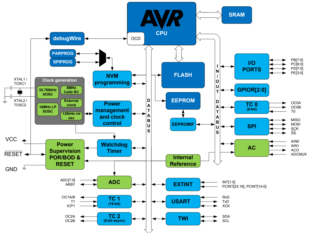
Figure 4-1. Block Diagram
