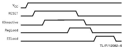
FIGURE 6. RESET Operation
