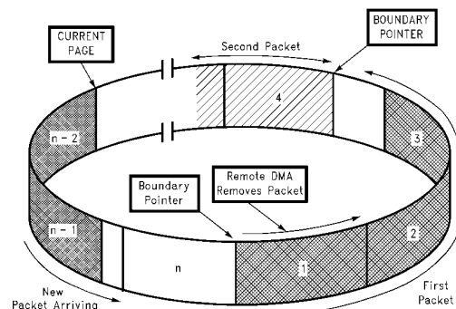
FIGURE 39. 1st Received Packet Removed by Remote DMA
