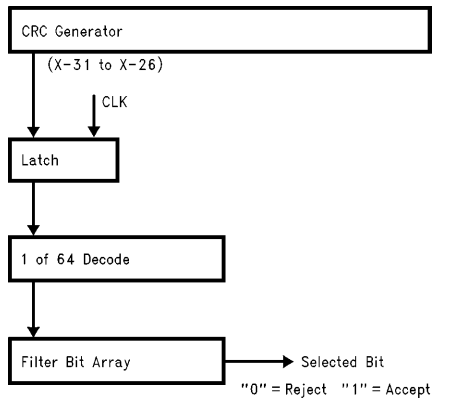
FIGURE 25. Multicast Addressing
