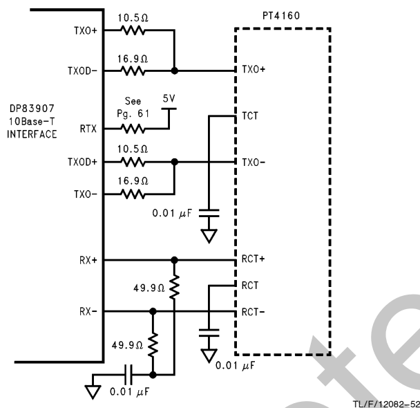
FIGURE 16b. Circuitry to Connect DP83907 to Twisted Pair Cable with Internal Filter
