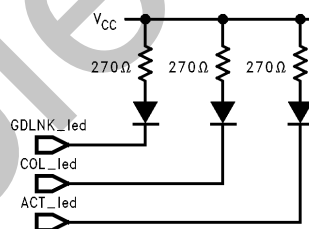
FIGURE 17. Typical DP83907 LED Connection
