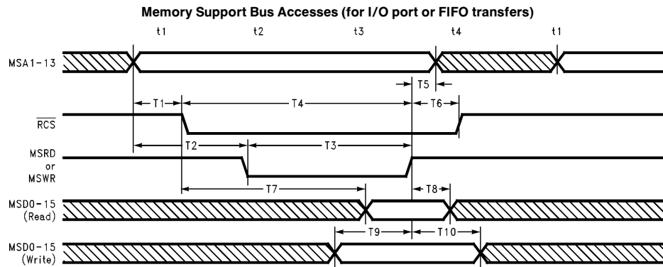
MEMORY SUPPORT BUS ACCESSES (for I/O Port or FIFO Transfers)
