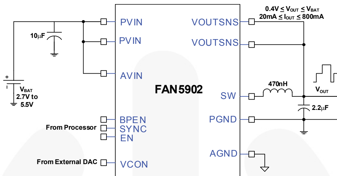
Figure 1. FAN5902 Circuit
