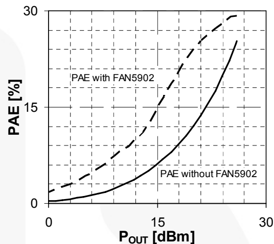
Figure 6. Comparison of RFPA Power Added Efficiency with and without FAN5902
