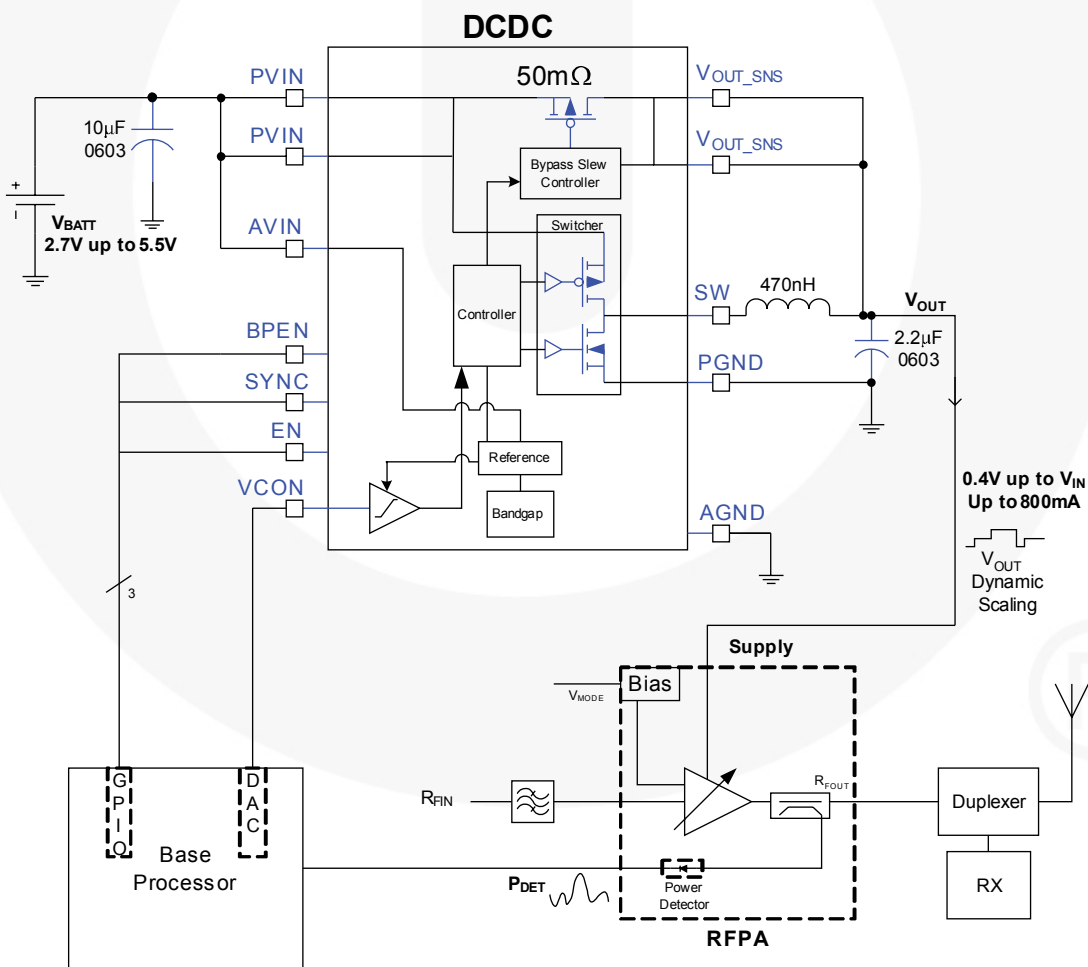
Figure 2. Typical Application
