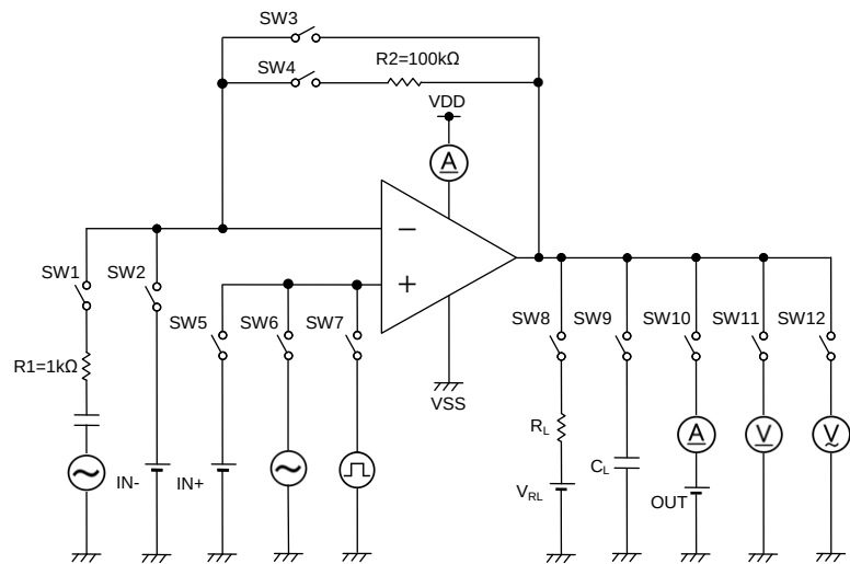
Figure 25. Test Circuit 2
