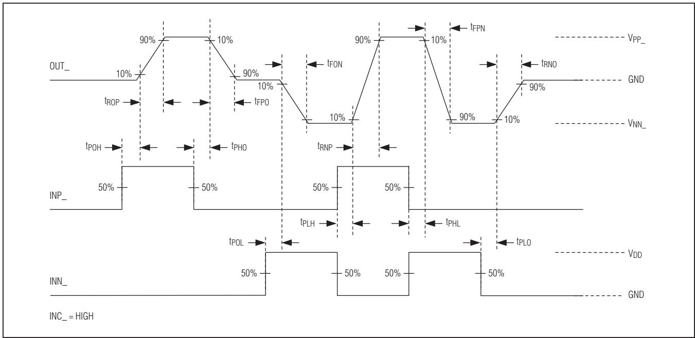
Figure 1. Detailed Timing ( R_L = 100\Omega , C_L = 100pF )
