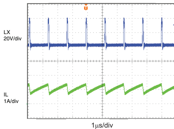
Switching Waveform ( V_{IN} = 5V , Full Brightness)
