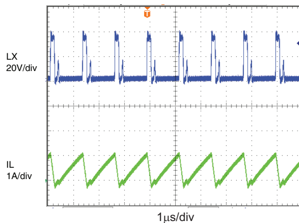
Switching Waveform ( V_{IN} = 25V , Full Brightness)
